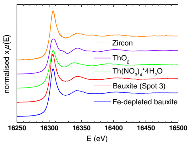
Fig. 5. Th L III -edge XAFS spectrum (bulk) of Fe-depleted diasporic Greek industrial bauxite (processing using the Athena software [12]), together with μ-XAFS spectrum from Spot 3, in comparison with spectra of reference materials: Th(NO 3 ) 4 ·4H 2 O, ThO 2 and zircon (ZrSiO 4 ).
