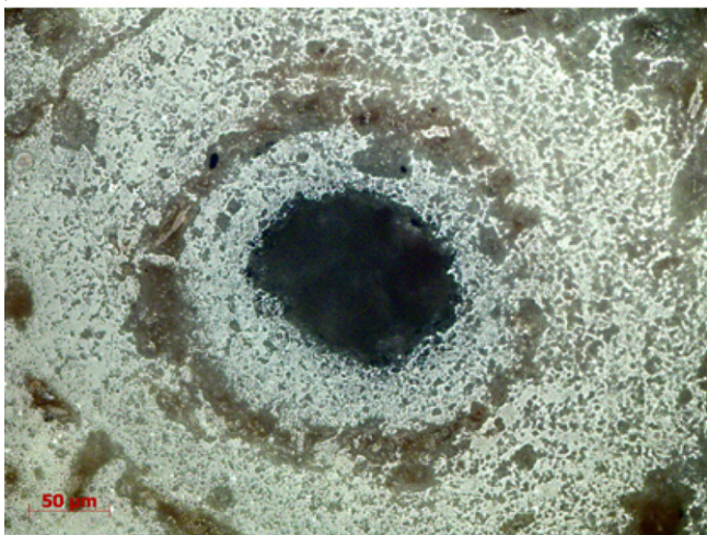
Fig. 1. Polished-section of Fe-depleted diasporic Greek industrial bauxite sample (upper) and detail of pisolith in the optical microscope (lower) prior to the \mu -XRF and \mu -XAFS measurements in the SUL-X beamline of ANKA.
